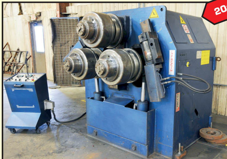
FACCIN 5" X 5" X .59" HYDRAULIC ANGLE BENDING ROLL
