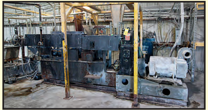
PRODEX 100 HP EXTRUDER
