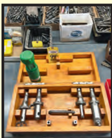
R-8 COLLET TOOLING SET
