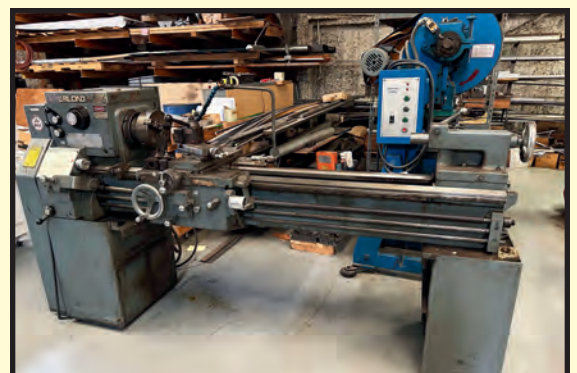
16" X 60" LEBLOND REGAL ENGINE LATHE
