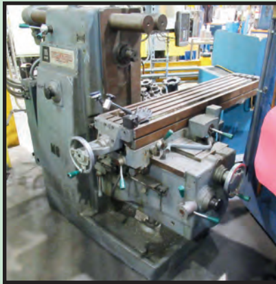
KEARNEY & TRECKER HORIZONTAL MILL
