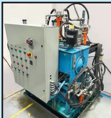
OIL-FLOW SKID
